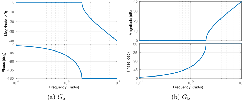
Figure 3.33: Magnitude and phase frequency responses for the two wave transfer functions
