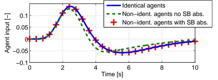
Figure 7: The comparison of the inputs to the fourth agent for three different multi-agent systems. The label 'SB abs.' stands for the soft-boundary absorber described by (67).
