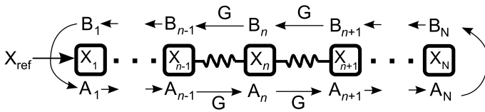
Figure 2: Scheme of a multi-agent system with a path-graph topology. The squares are agents with local dynamics described by (3) and (5). The virtual connections between the agents, which are created by the local control law, are illustrated by springs. All agents are identical.
