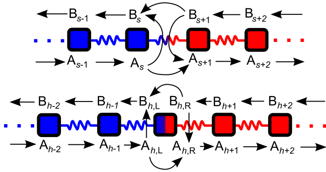
Figure 3: Scheme of a multi-agent system with the soft and hard boundaries in top and bottom, respectively. The blue and red squares are agents with the WTFs of G(s) and H(s) , respectively, defined in (23) and (26). The virtual connections between the agents are illustrated by springs. The blue-red spring is the soft boundary and the blue-red square is the hard boundary.
