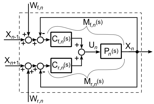
Figure 1: The model of n th agent.
