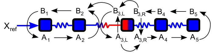
Figure 9: Scheme of the complex boundary between 2nd and 3rd agents composed of the soft and hard boundaries next to each other in a multi-agent system described by (88)-(89). The blue arrow in front of the first agent represents the input to the system.
