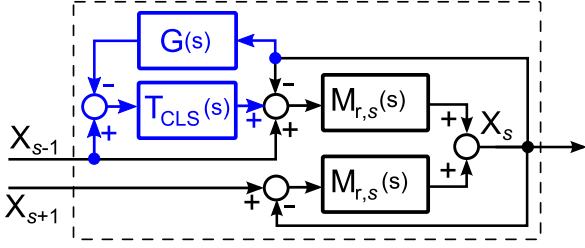
Figure 4: The model of s th agent with the left-side absorbing controller (highlighted in blue), where T_{CLS} = G(s)(G(s) - H(s))/(1 - G^2(s)) from (67). The front and rear ATFs are identical since, for now we assume only one soft boundary in the system as at the top of Fig. 3.
