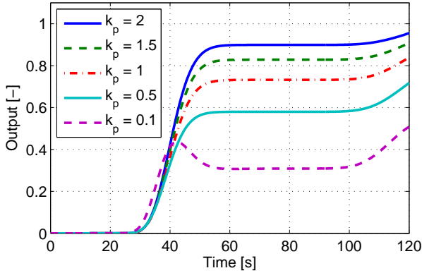
Figure 8: The numerical simulations of a multi-agent system described by (85)-(86) for different values of k_p . The output of the 41 st agent is shown.
