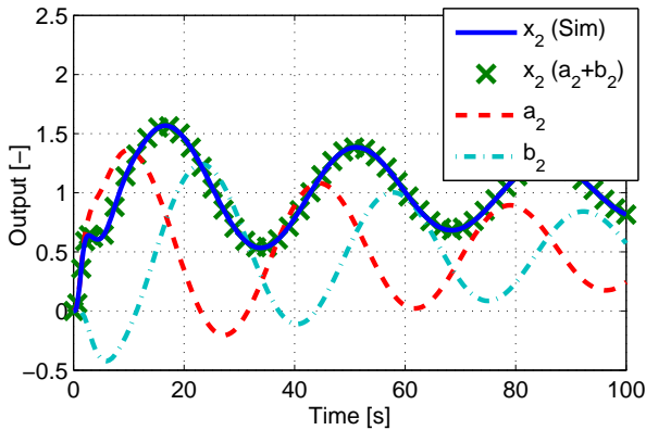
Figure 10: The comparison of the outputs of the 2nd agent simulated by the state-space approach using (88)-(89) (solid line) and that computed by the WTF approach using (90)-(93). The response to the step change of x_{\text{ref}}(t) is shown.
