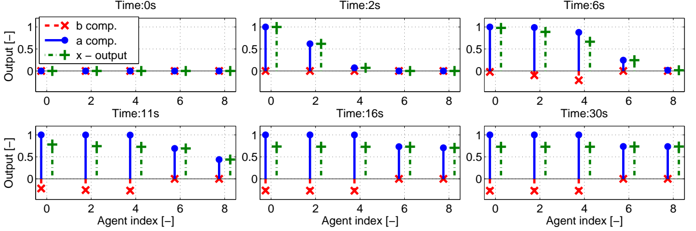
Figure 5: Simulation of the wave propagating in a multi-agent system with the path-graph topology defined by (83)-(84). At the beginning, t = 0^+ s, outputs of all agents are 0 except x_{\text{ref}}(t) , which is changed from 0 to 1. At intermediate times, the wave travels to the soft boundary, where it is transmitted and attenuated by a factor \kappa_{aa} and reflected by a factor \kappa_{ab} . As the wave propagates back to the first agent, it forces the first four agents to change their output by \kappa_{ab} (negative value in this case). The waves are absorbed on 1st and 8th agents by the wave-absorbing controllers. The blue circles and red crosses represent a(t) and b(t) components of the wave, respectively. The green plus signs stand for the outputs of the agents. The 0th agent is the input to the system from (13), i.e. X_0(s) = W_{f,1}(s) , A_0(s) = X_{\text{ref}}(s) and B_0(s) = GB_1(s) .
