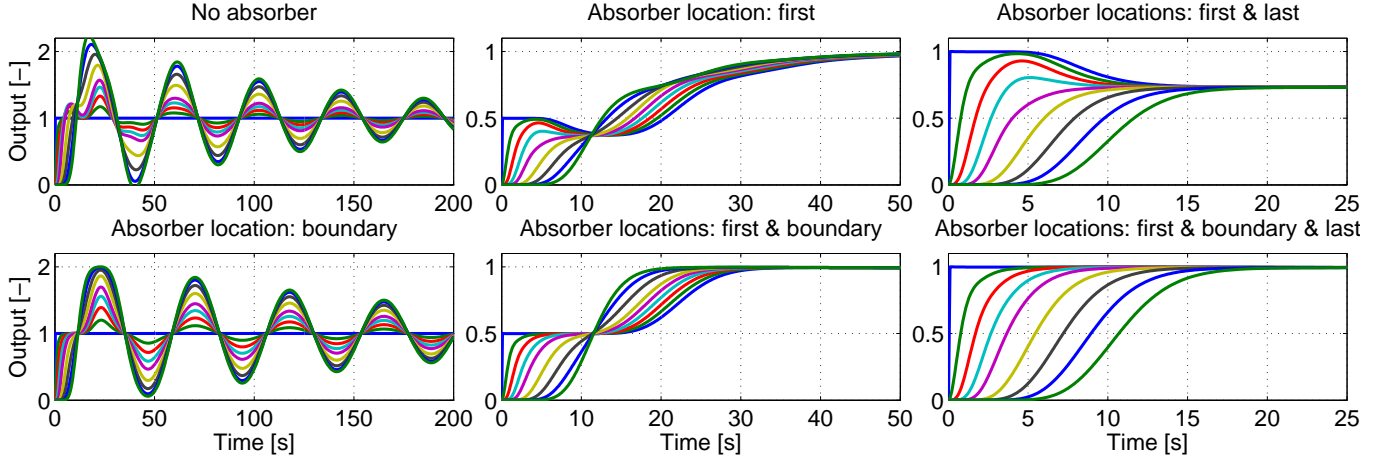
Figure 6: The performance comparison of individual control strategies for a multi-agent system with the soft boundary. The multi-agent system is defined by (83)-(84) with x_{\text{ref}}(0) = 1 and x_i(0) = 0 for i = 1, 2, \dots, N . The step responses of six individual control strategies are compared. The top-left: the system with no absorber; top-middle: the system with the absorber implemented on the first agent; top-right: the system with the absorbers implemented on the first and rear-end agents. In the bottom panels, the soft-boundary absorber between the agents 4 and 5 is additionally implemented.
